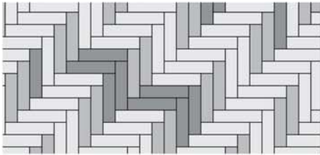
Plaza Paving Option #1 - Herringbone
